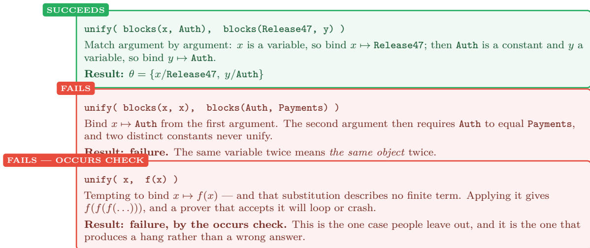
Figure 12.2: Three unification problems. The third is why every implementation needs an occurs check, and why many production Prolog systems omit it for speed and document the risk.
